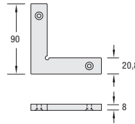
Z 966 Eckverbinder OCTAfabric Aluminium
